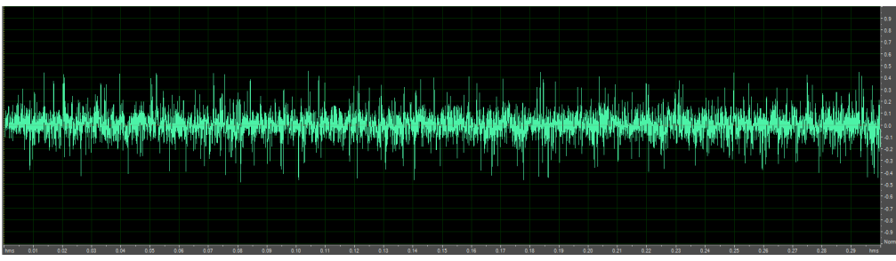
Figure 5 FM noise without carrier (below threshold) with clicks (after deemphasis 50μs)
